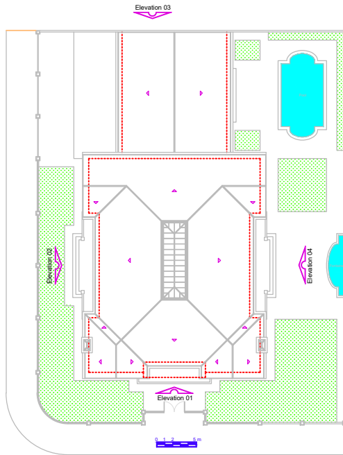
Roof Plan
